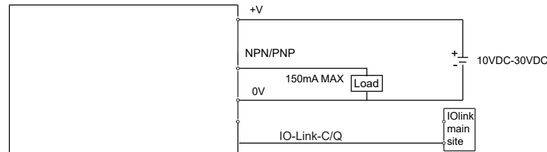
Wiring diagram (PNP)
